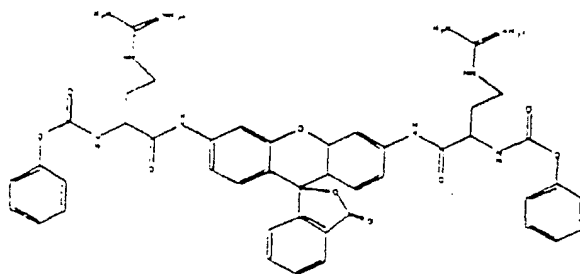
Rhodamine protease substrate.
